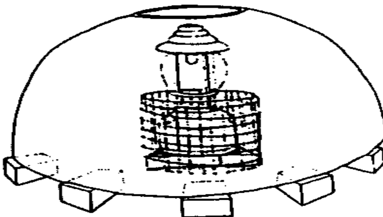
FIGURE 81: KEROSENE BROODER
