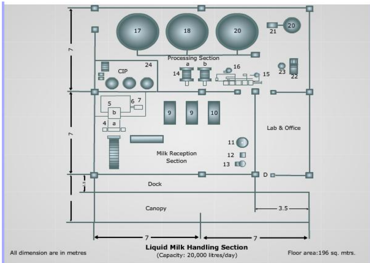
Fig. 16.1 Liquid Milk Handling Section
