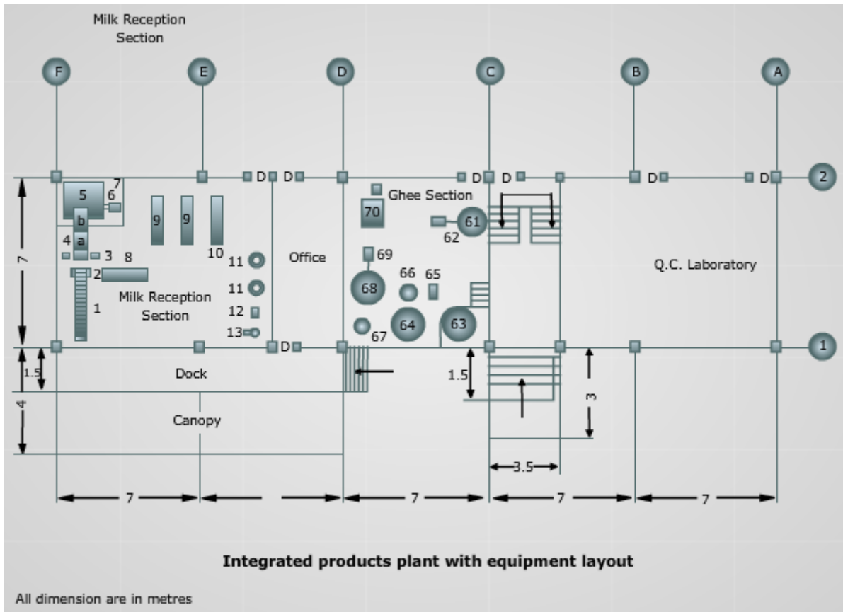
Fig. 21.3 Integrated product plant with equipment layout
