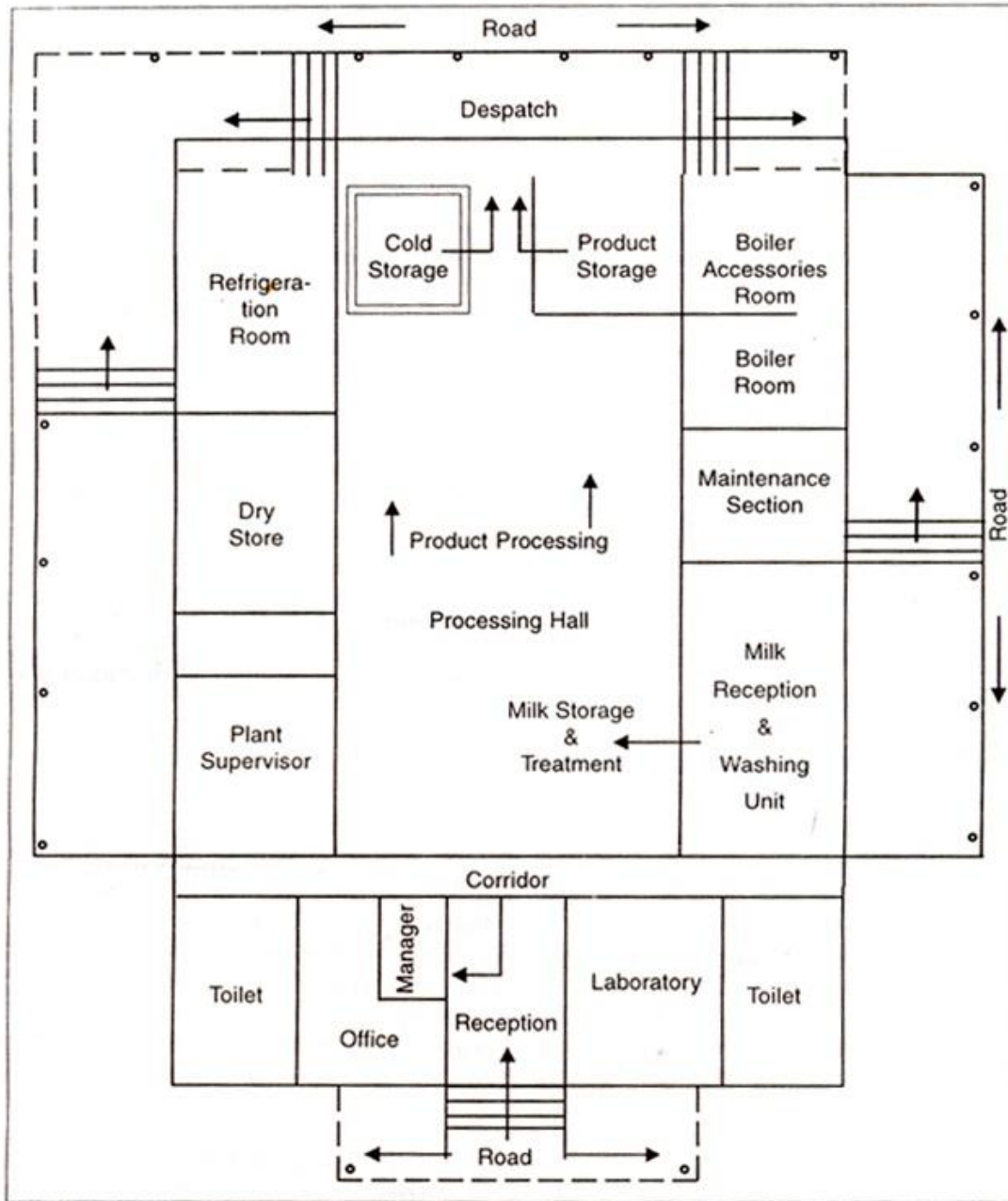
Fig. 24.1 Concept for layout of dairy plant
