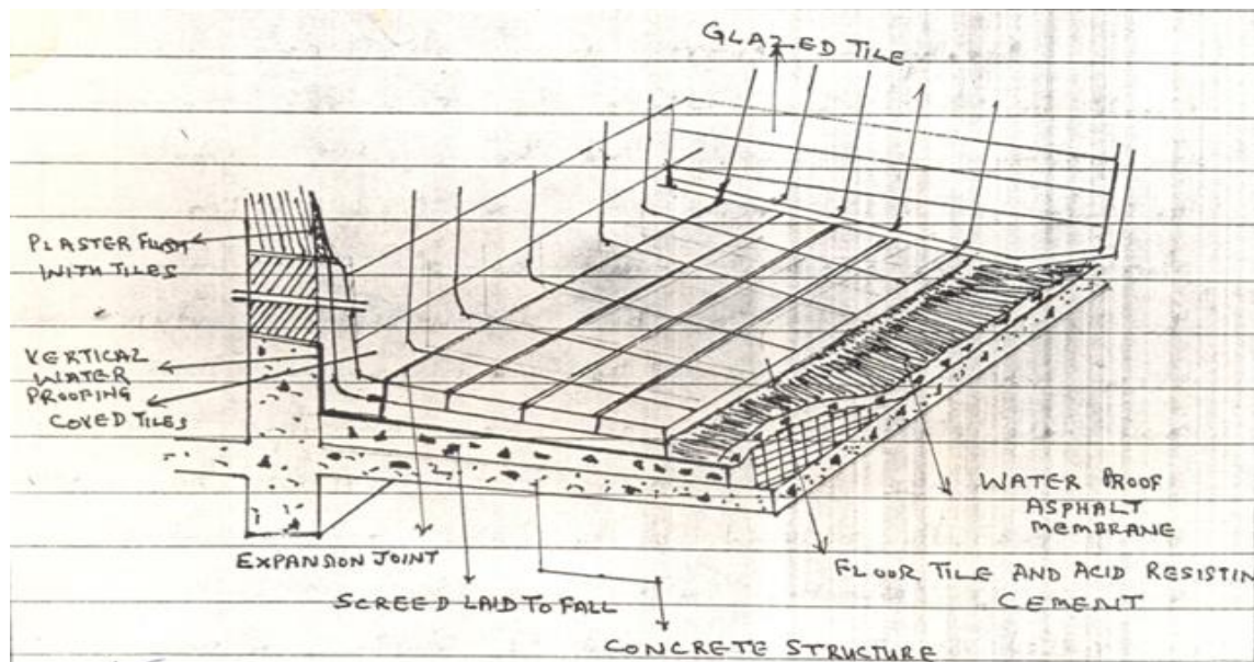
Fig. 28.1 Floor Construction
