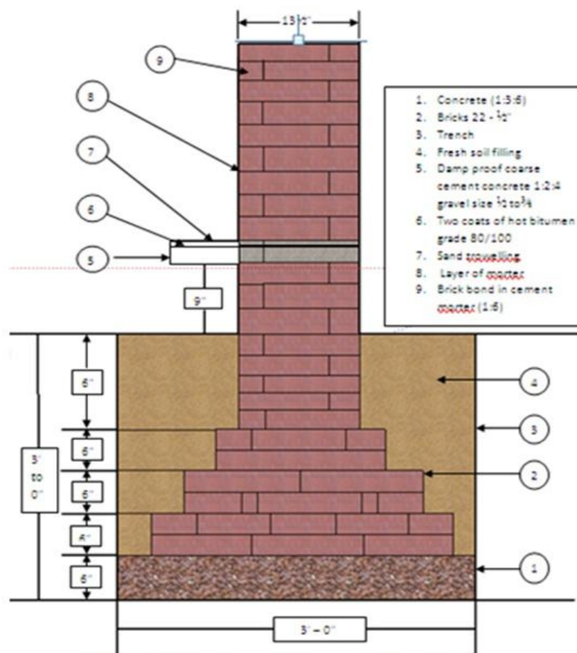
Fig. 29.1 Section of stepped foundation
