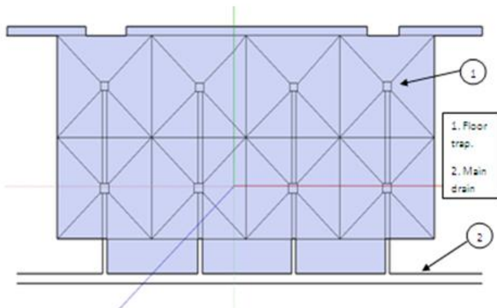
Fig. 30.2 Drain layout of a large milk processing room
