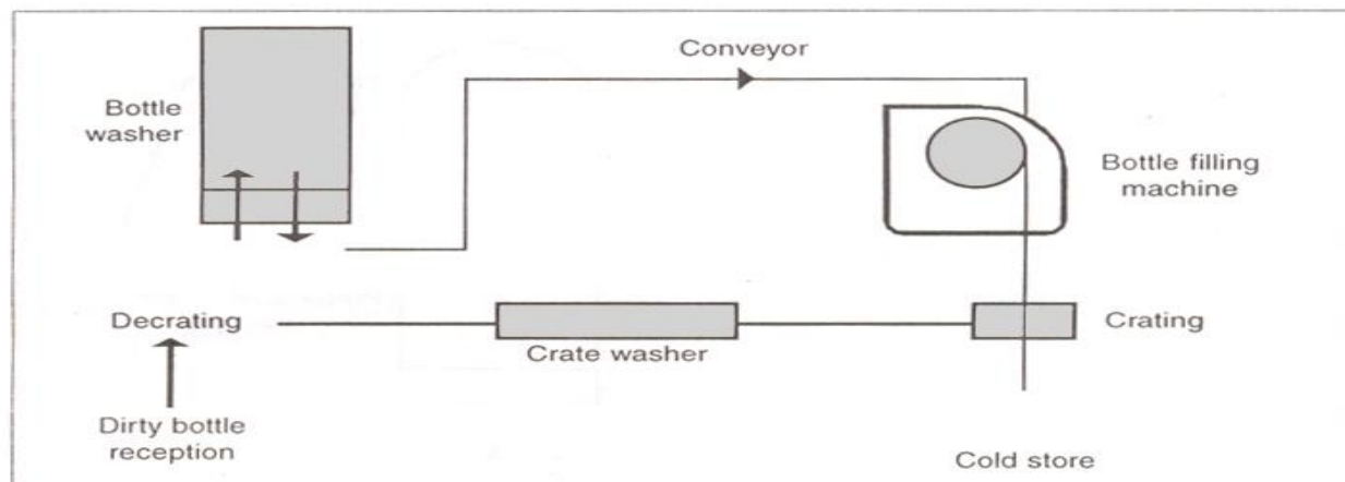
Fig 19.9 Arrangement of bottling section using come back type washer
