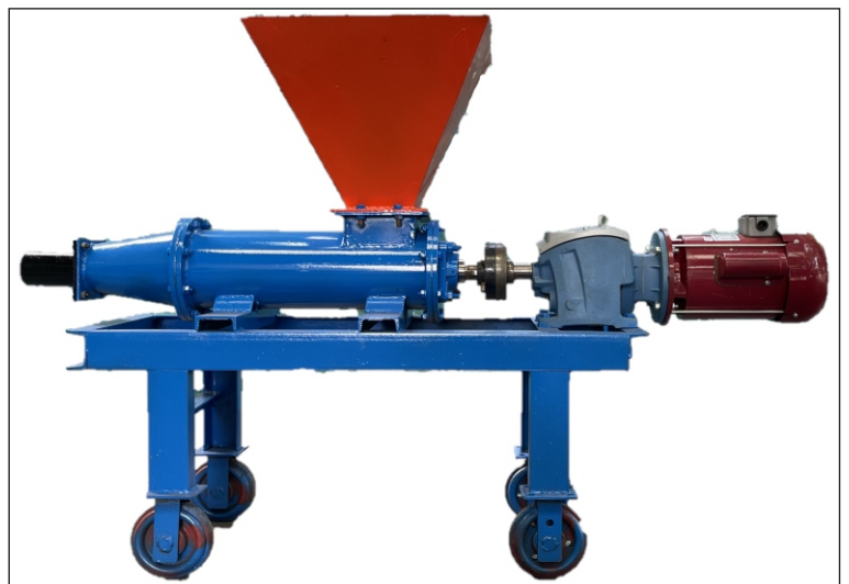
Cow Dung Log Making Machine
